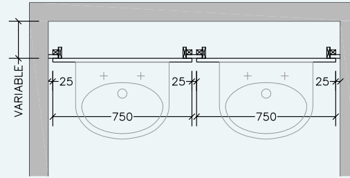
PLAN LAYOUT
