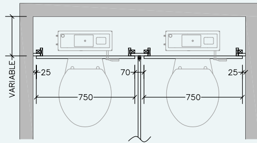
PLAN LAYOUT
