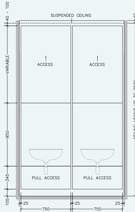
FRONT ELEVATION
