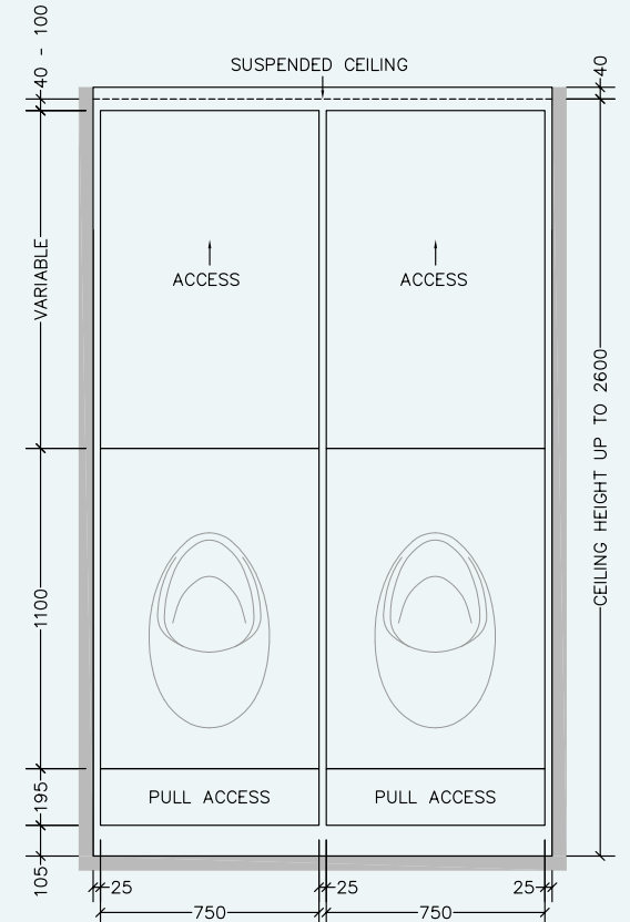
FRONT ELEVATION
