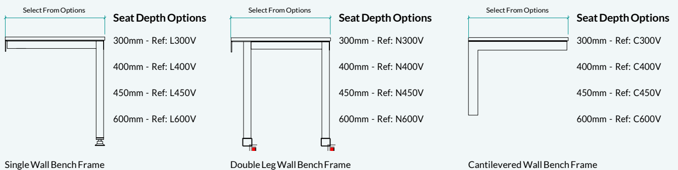
Single Wall Bench Frame
